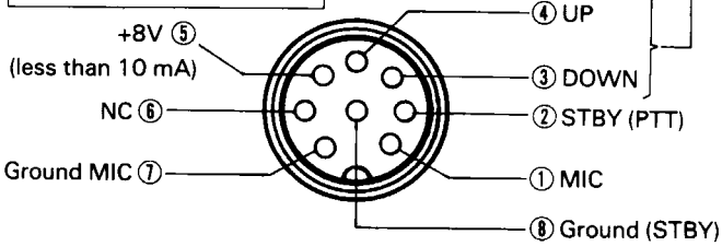
MIC connector < Front panel view >
